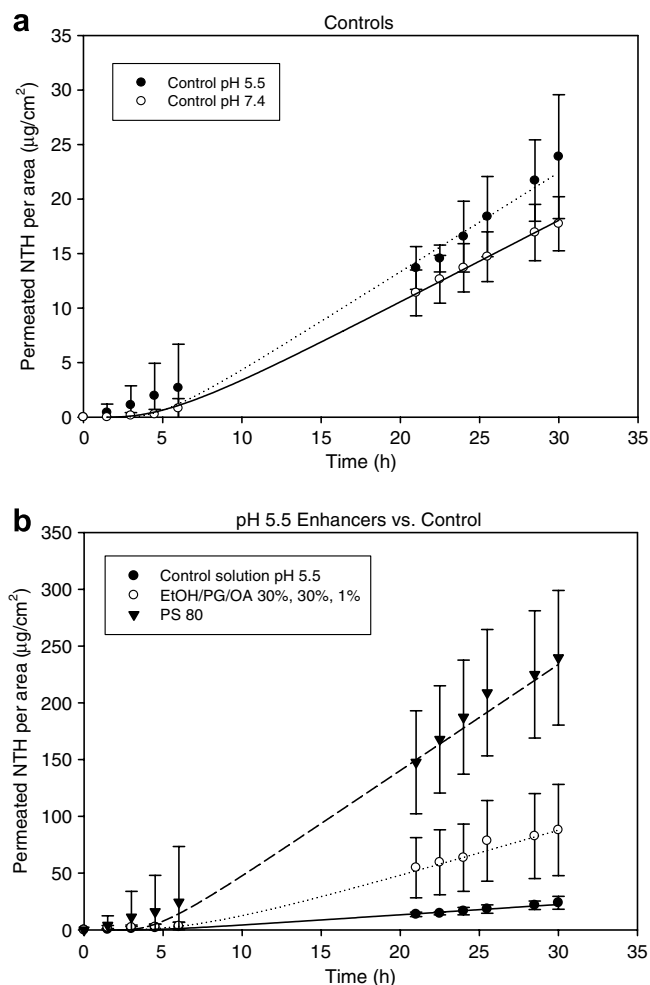
Fig. 1. Permeation profiles (mean \pm SD) of NTH across human epidermis from different solvent systems at different pHs (a) and pH 5.5 with penetration enhancers (EtOH, ethanol, PG, propylene glycol, OA, oleic acid, PS 80, polysorbate 80) (b).
